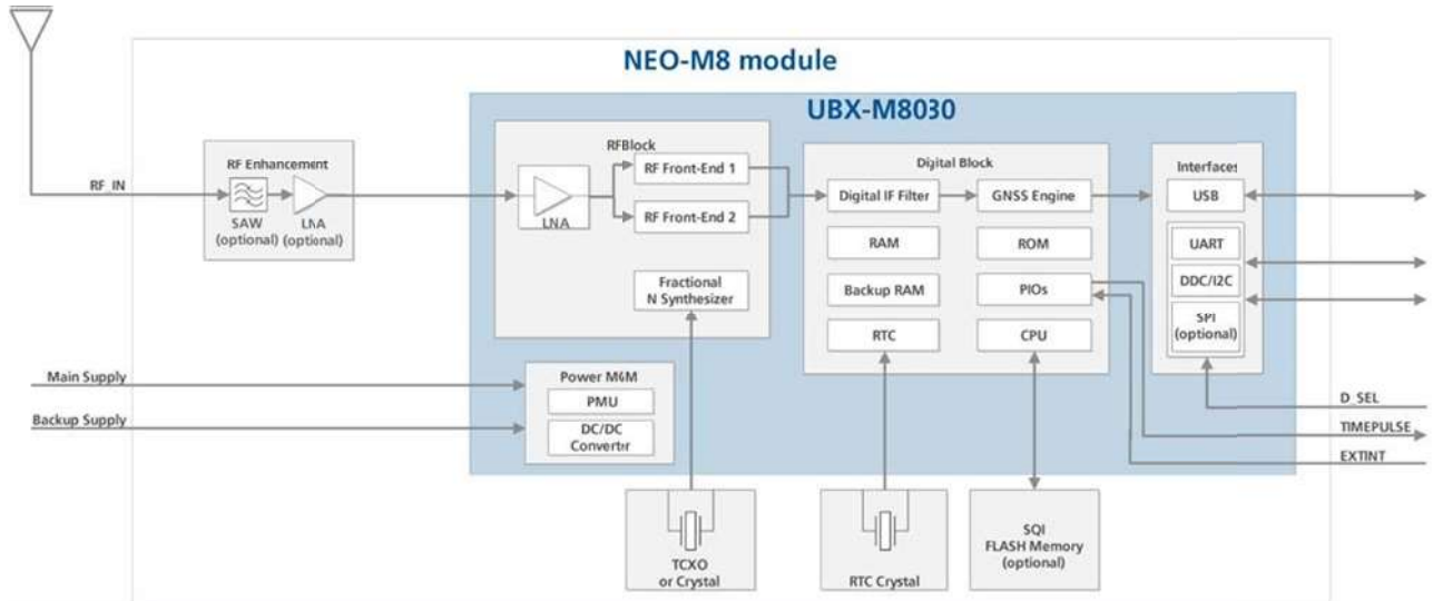
Figure 1: NEO-M8 block diagram
