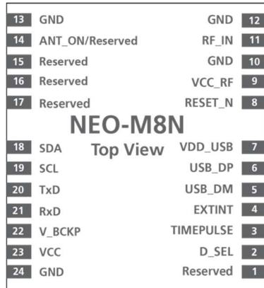
Figure 2: Pin Assignment
