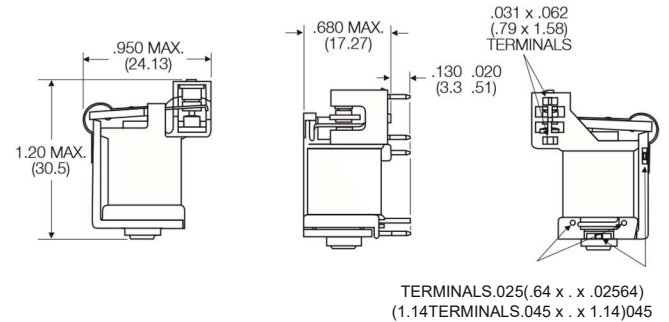
Terminal assignment Bottom view on pins
