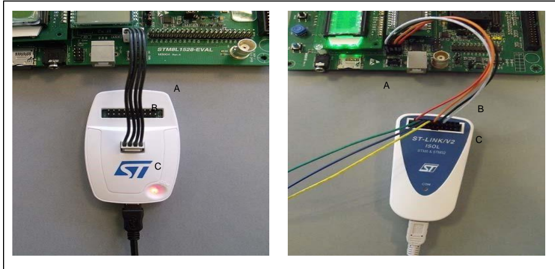
Figure 7. Low-cost connection
