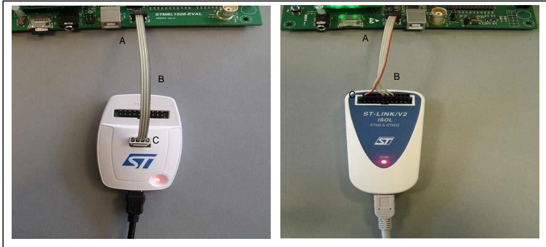
Figure 5. ERNI connection
