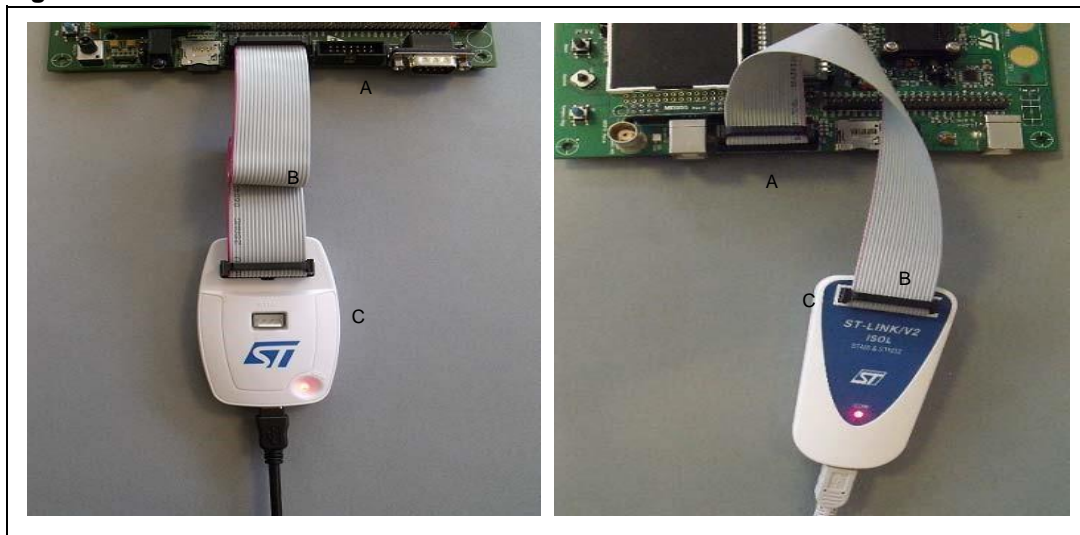
Figure 9. JTAG and SWD connection
